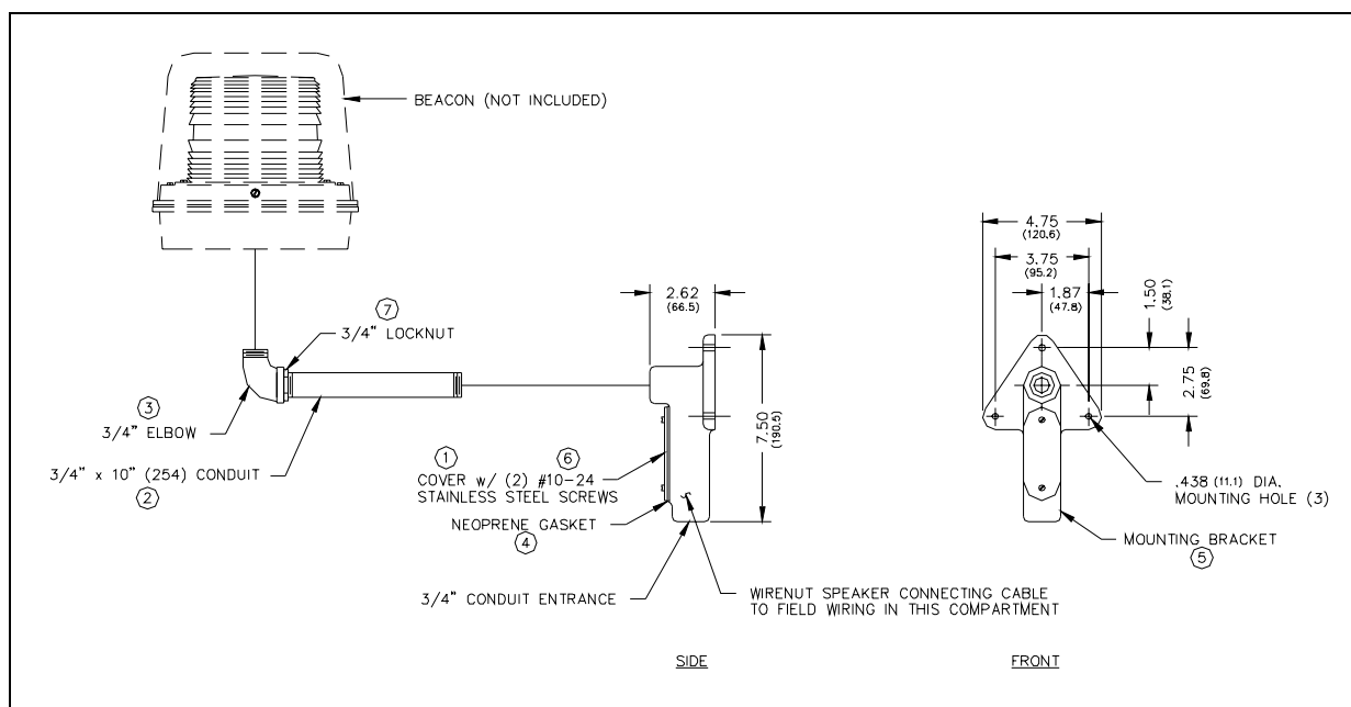
Figure 1. Speaker Mounting Details
