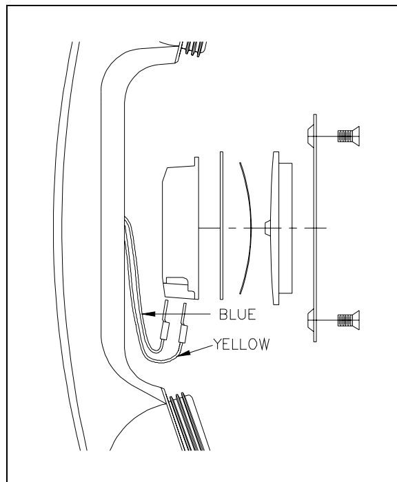
Figure 1. Handset Assembly with Pressbar
