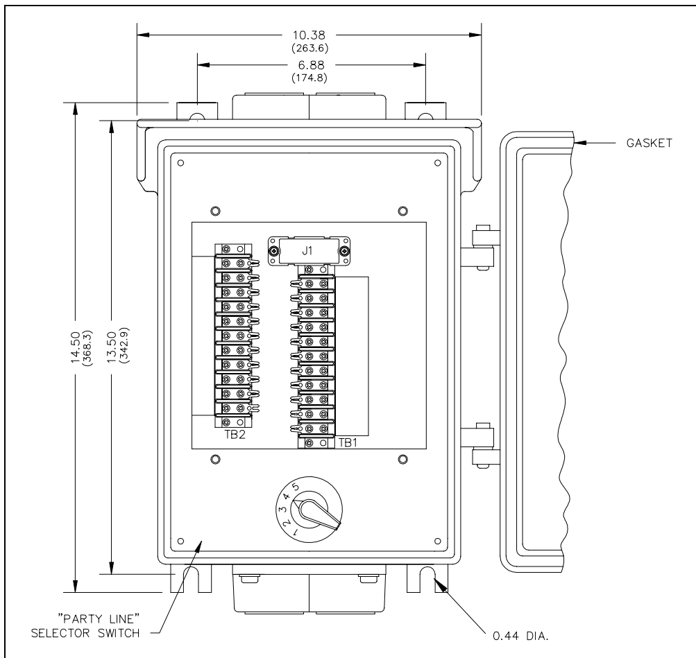
Figure 1. Model 7325-106 Enclosure Mounting Details
